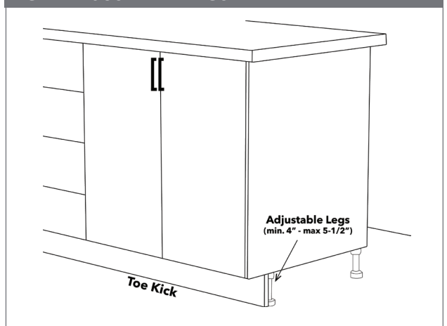
FIG 7: ADJUSTABLE LEGS
